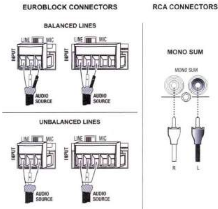
Figure 2.4.1 Input Wiring
