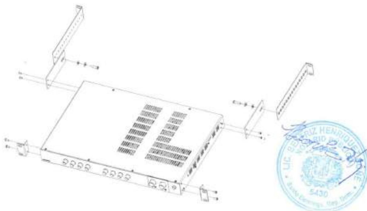
Figure 2.2.5 Rack Mounting Full Rack Mixer Amplifier
