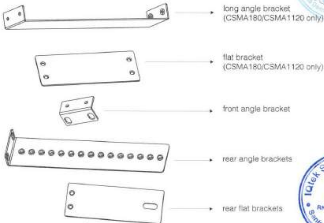
Figure 2.2.2 Mounting Kit
