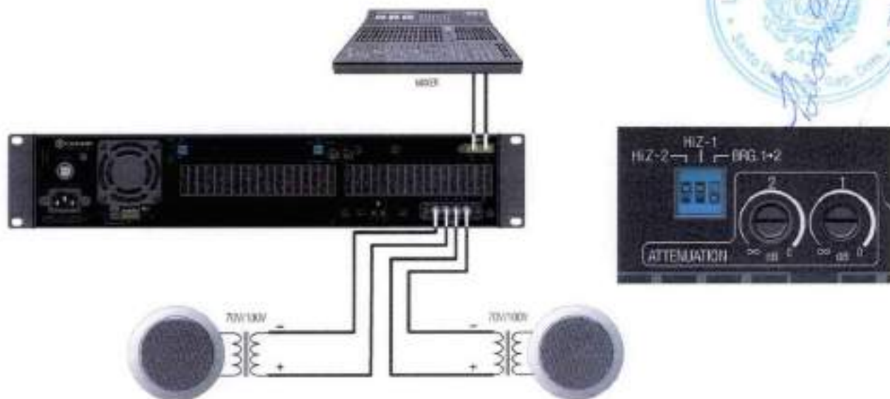
Figure 8 System Wiring for 70V/100V Operation
