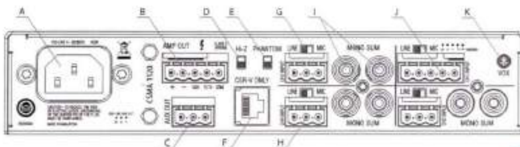
Figure 1.3 Rear View - CSMA 1120
