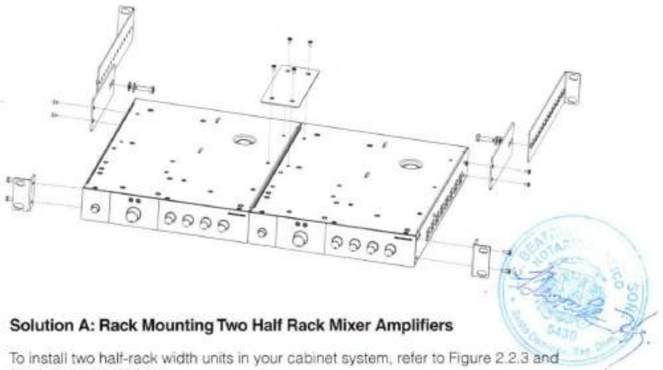
Figure 2.2.3 Rack mounting of two half rack Mixer units.
