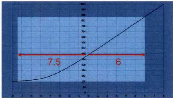
13.5 stop Wide Dynamic Range
